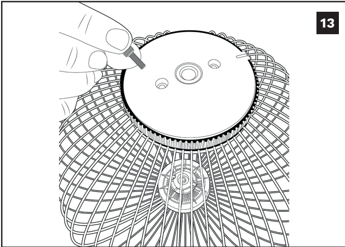
Insert the 2 x M4 screws into the two holes and tighten with allen key provided.
