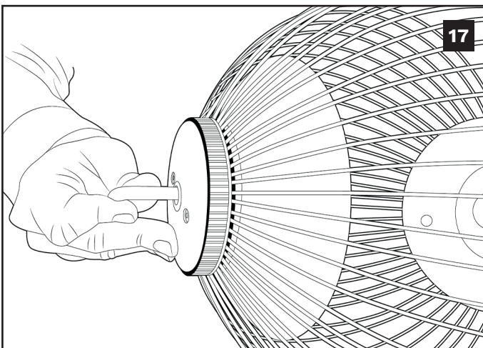
Take the cage mounting bracket and line up the prongs at the bottom with holes in the end caps as shown. To aid in achieving this squeeze the ends of the cage together
